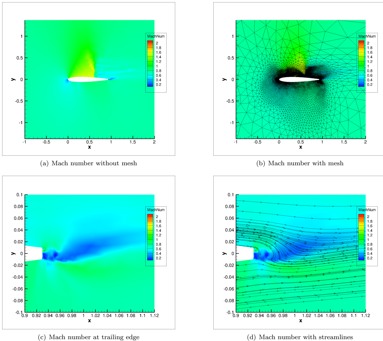
Figure 19. 16th and final adaptation cycle for transonic blunt trailing edge test case with virtual mesh error estimation
