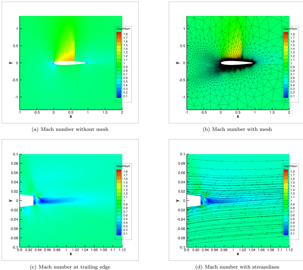
Figure 23. 16th and final adaptation cycle for transonic blunt trailing edge test case with embedded mesh error estimation
