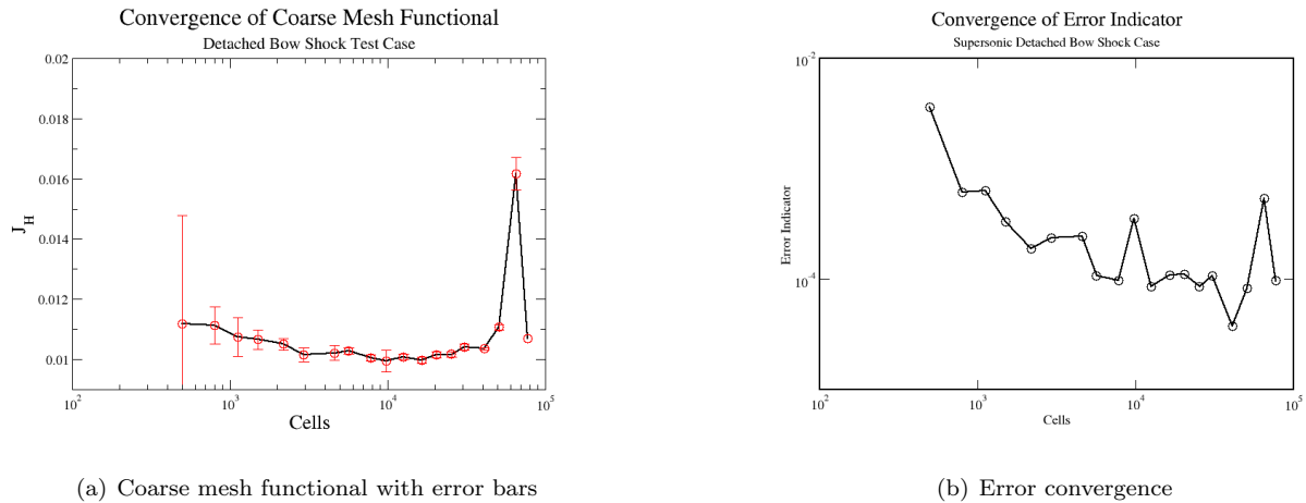
Figure 11. Functional and error estimate convergence for supersonic detached bow shock test case with embedded mesh error estimation
