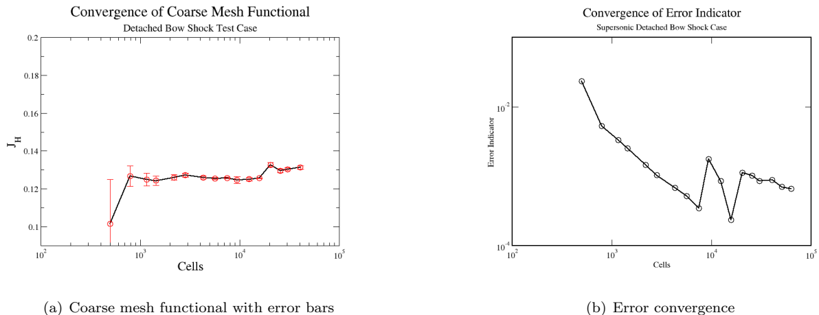
Figure 7. Functional and error estimate convergence for supersonic detached bow shock test case with virtual mesh error estimation
