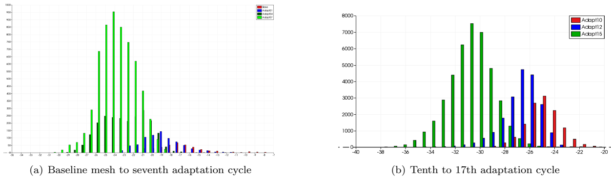
Figure 28. Error histograms for transonic blunt trailing edge case test case with embedded mesh error estimation and functional correction
