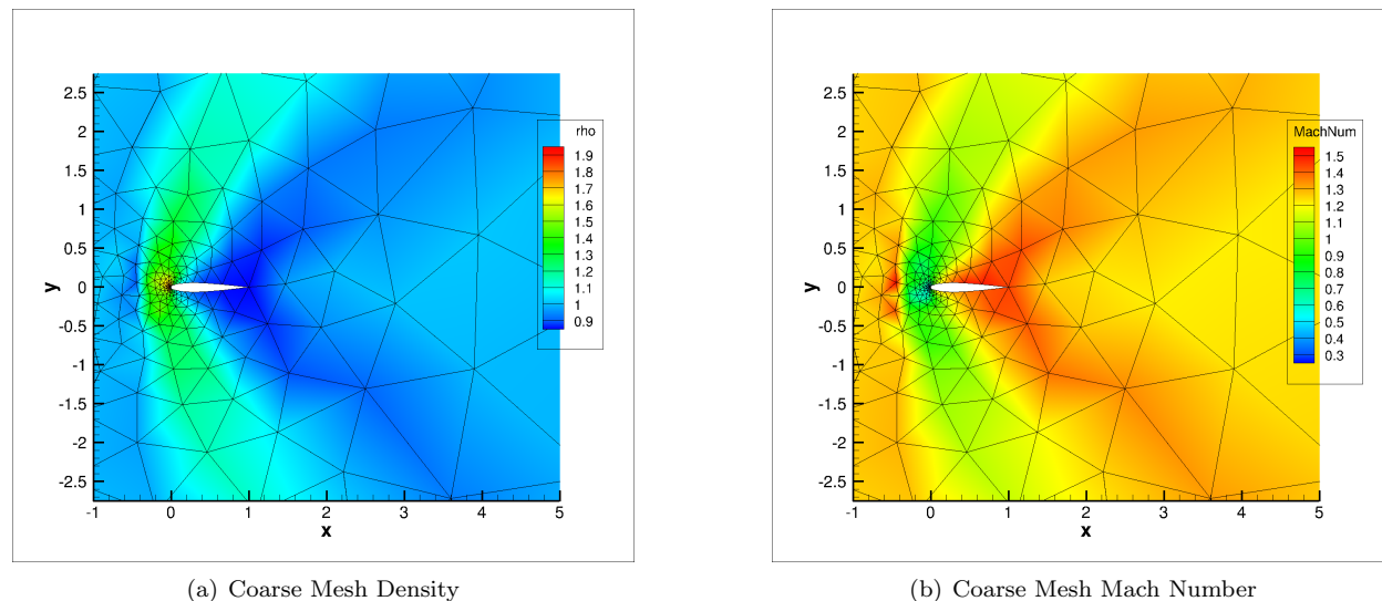
Figure 2. Coarse mesh for detached bow shock error estimation case
