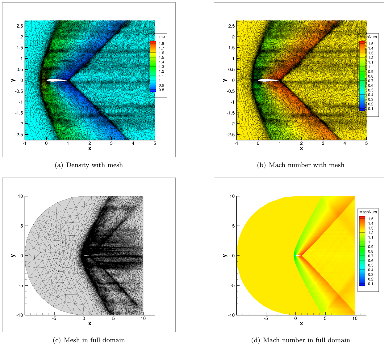
Figure 9. 18th and final adaptation cycle for detached bow shock test case with embedded mesh error estimation
