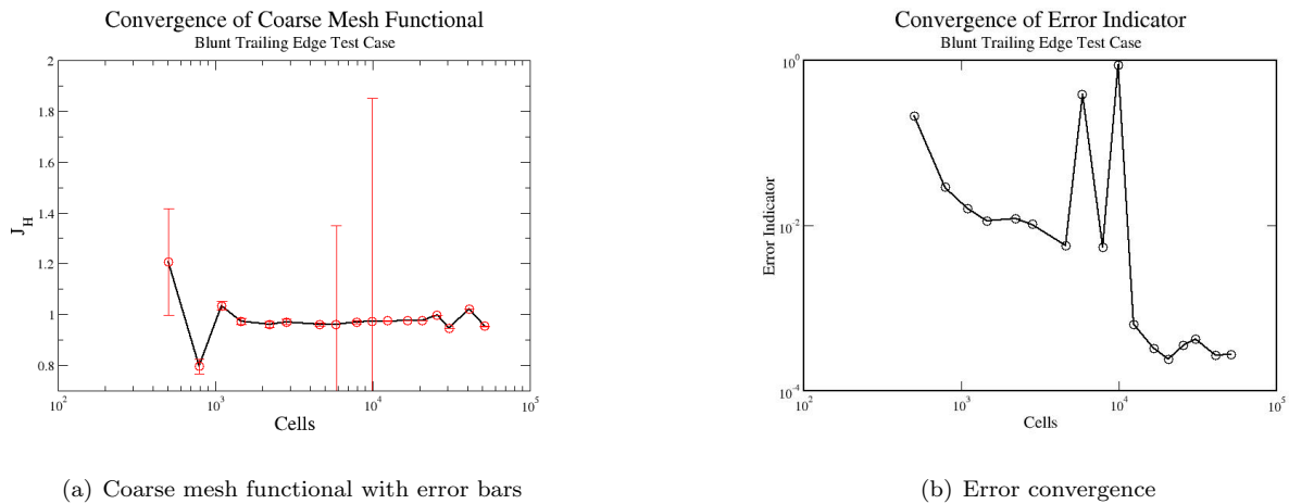
Figure 25. Functional and error estimate convergence for transonic blunt trailing edge test case with embedded mesh error estimation
