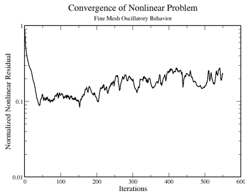
(a) Fine Mesh Convergence
