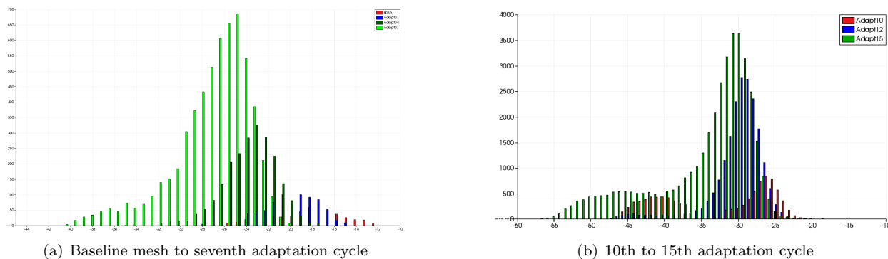
Figure 14. Error histograms for detached bow shock test case with embedded mesh error estimation and functional correction
