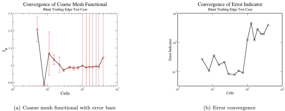
Figure 21. Functional and error estimate convergence for transonic blunt trailing edge test case with virtual mesh error estimation
