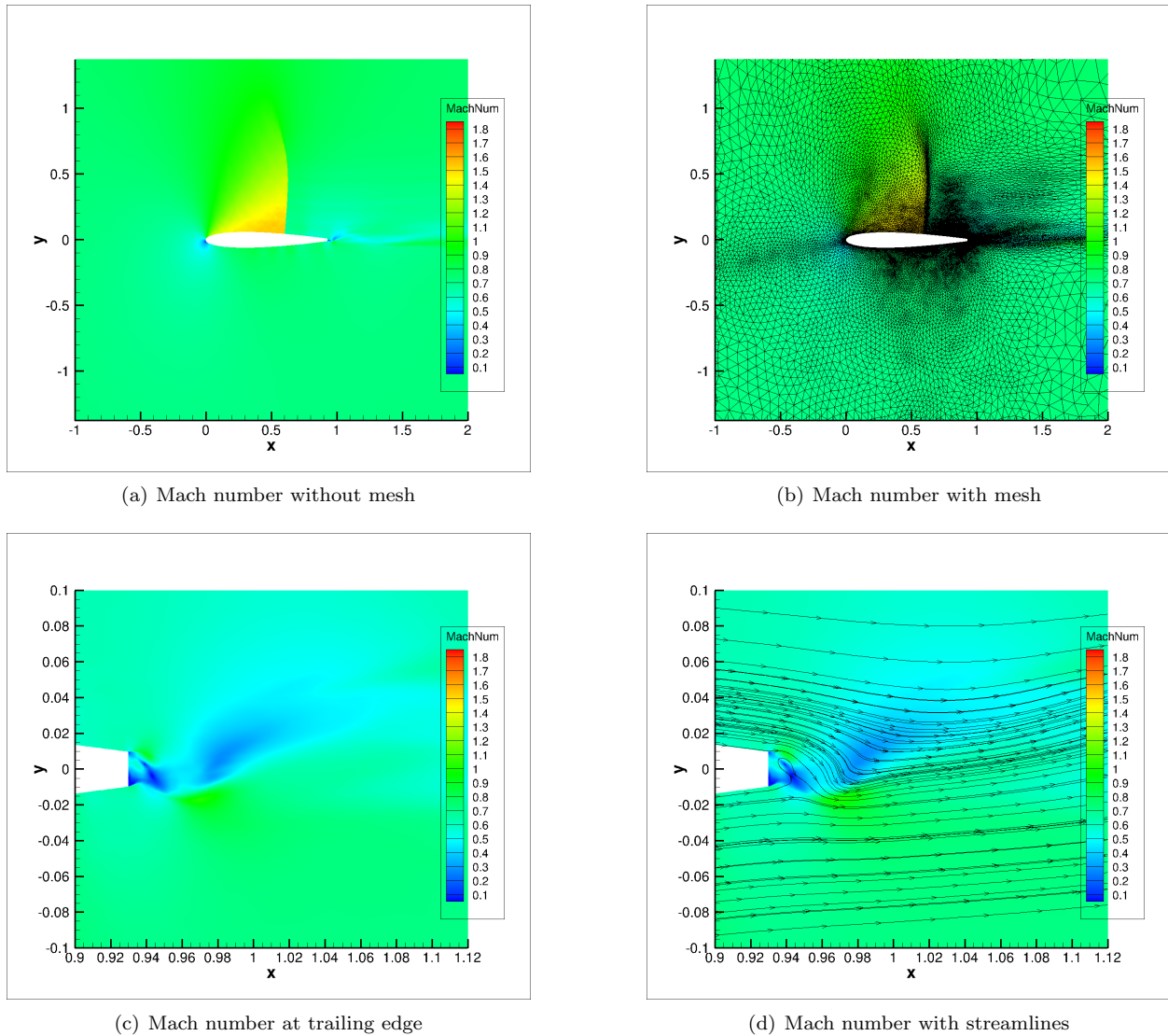
Figure 27. 16th and final adaptation cycle for transonic blunt trailing edge test case with embedded mesh error estimation and functional correction
