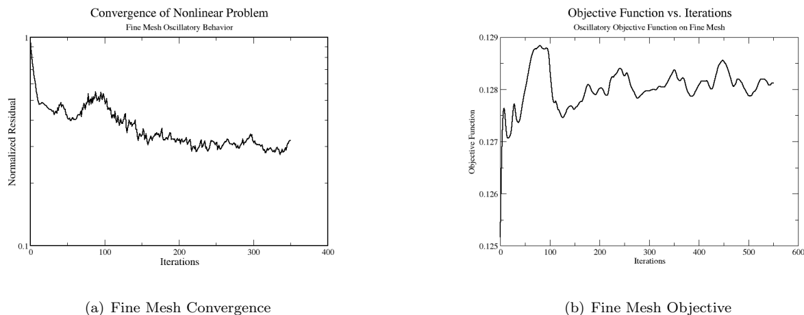
Figure 3. Objective and convergence behavior on final adapted mesh
