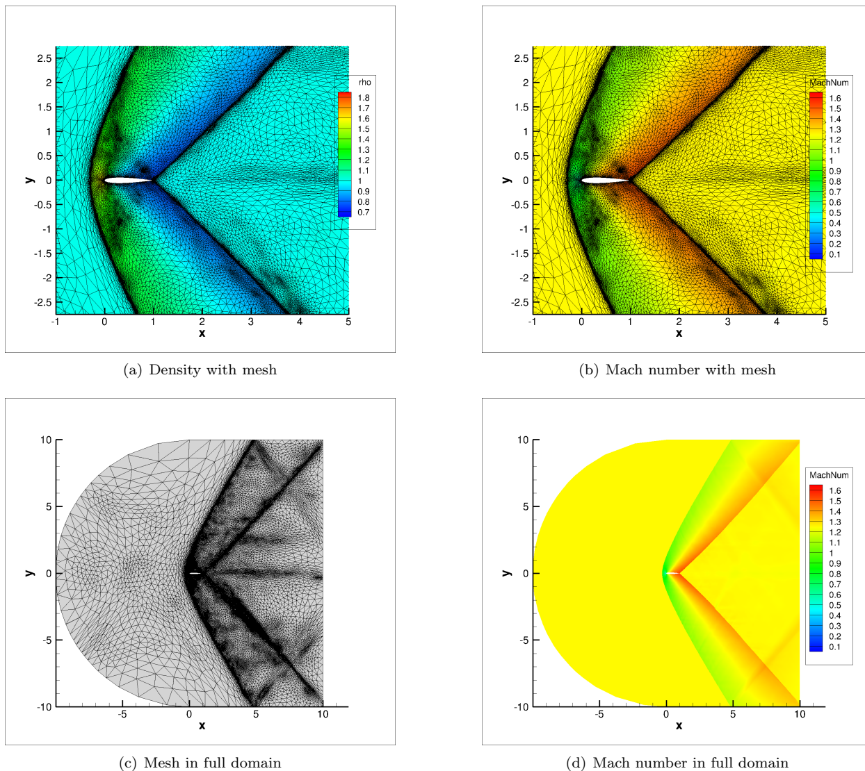
Figure 13. 18th and final adaptation cycle for detached bow shock test case with embedded mesh error estimation and functional correction
