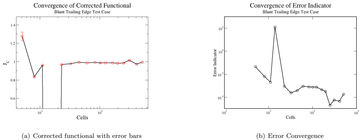
Figure 29. Corrected functional and error estimate convergence for transonic blunt trailing edge test case with embedded mesh error estimation and functional correction
