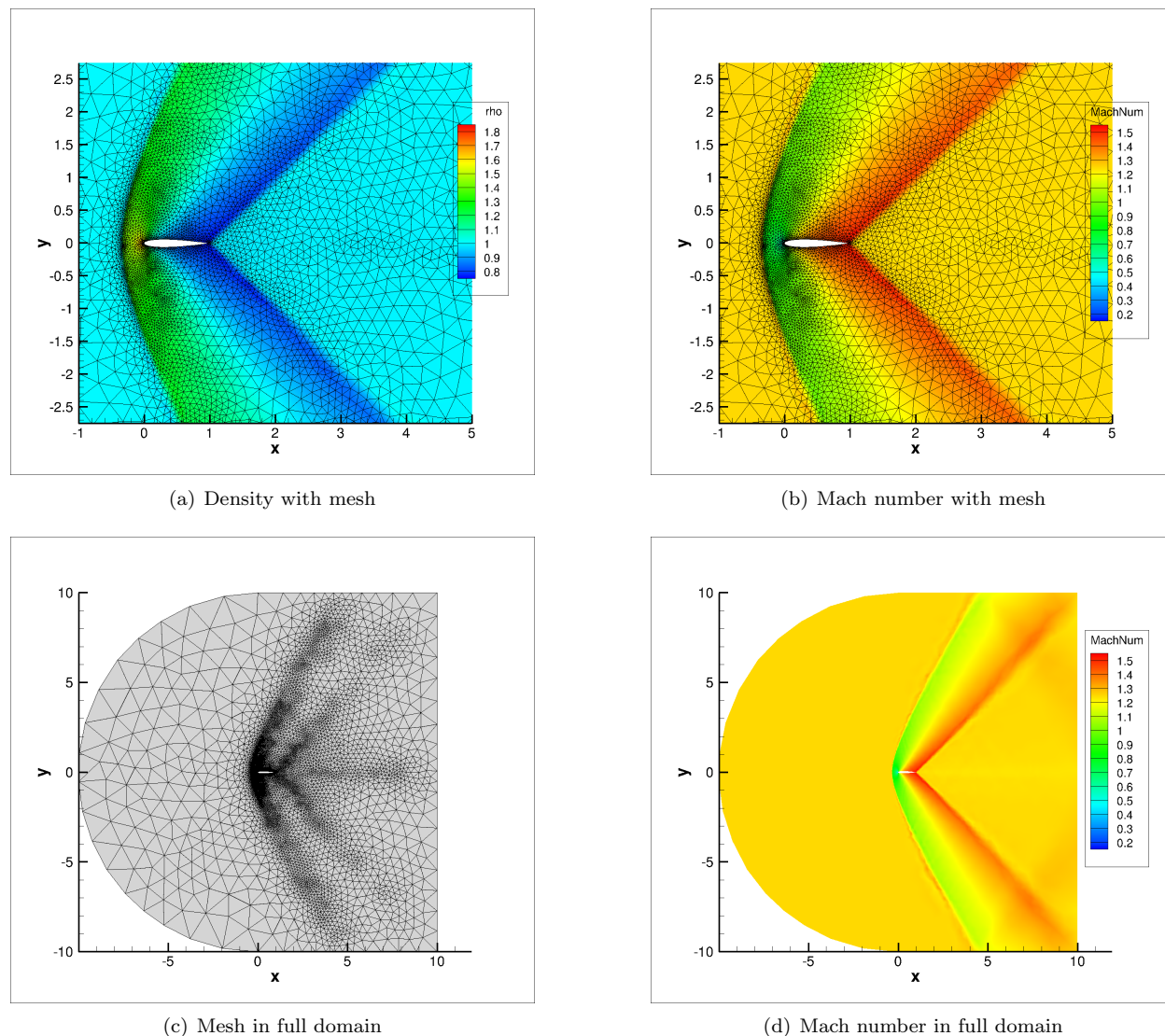
Figure 4. Tenth adaptation cycle for detached bow shock test case with virtual mesh error estimation (final isotropic mesh)
