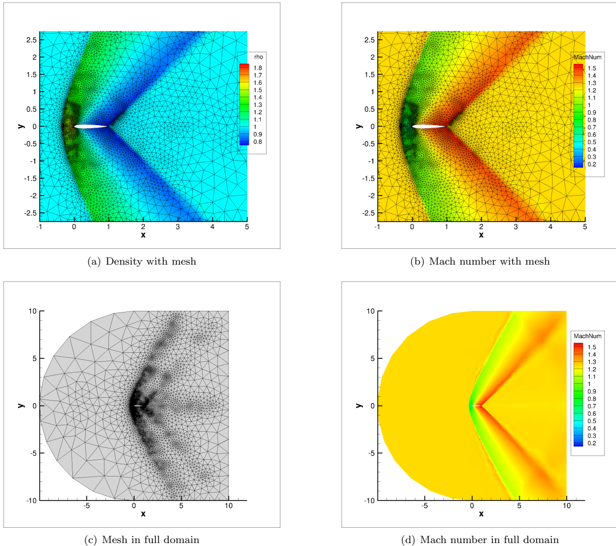
Figure 8. Tenth adaptation cycle for detached bow shock test case with embedded mesh error estimation (final isotropic mesh)
