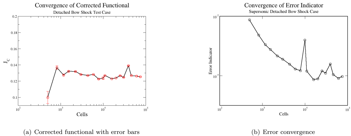
Figure 15. Corrected functional and error estimate convergence for detached bow shock test case with embedded mesh error estimation and functional correction
