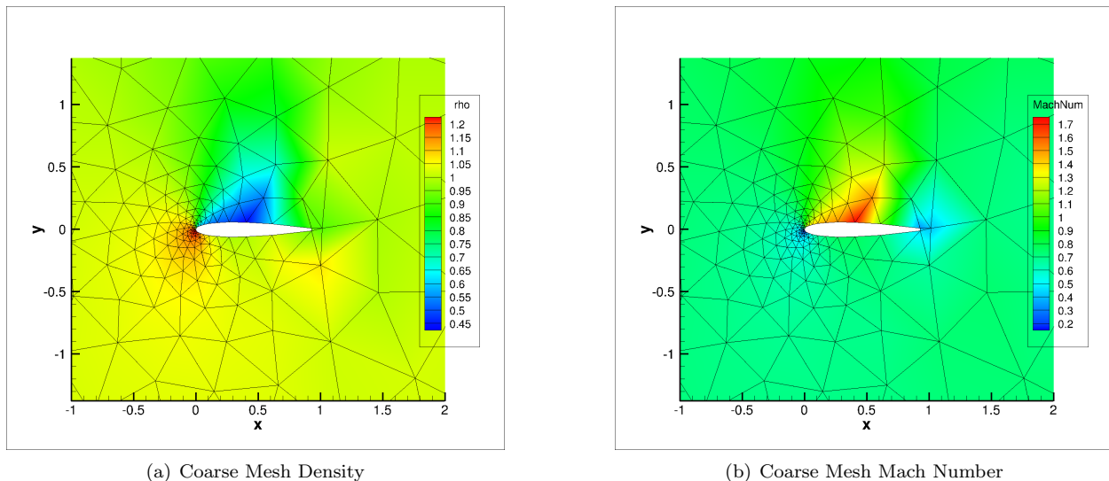
Figure 16. Coarse mesh for transonic blunt trailing edge error estimation case
