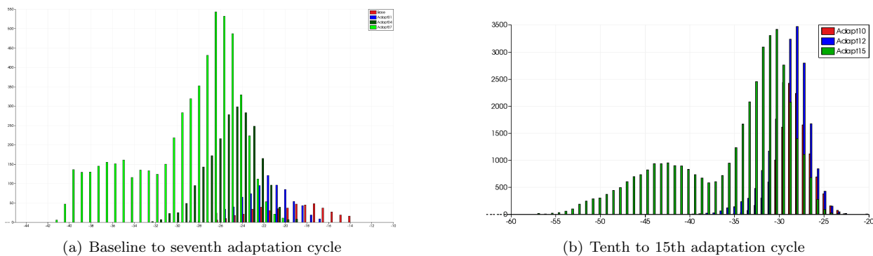
Figure 10. Error histograms for detached bow shock test case with embedded mesh error estimation
